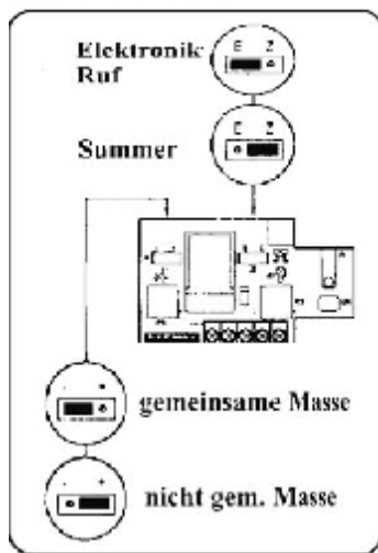
Jumper Positionen
